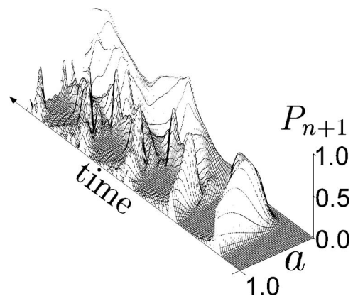
FIG. 1. The evolution of P_{n+1}(t) for the system of 30 spins for t \in [0, 150] .
