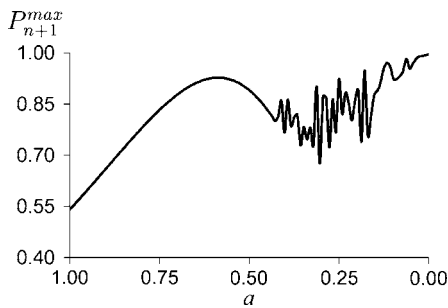
FIG. 3. The dependence of P_{n+1}^{\max}=\max\{P_{n+1}(t): t \in[0,20000]\} on a for the system of 30 spins.
