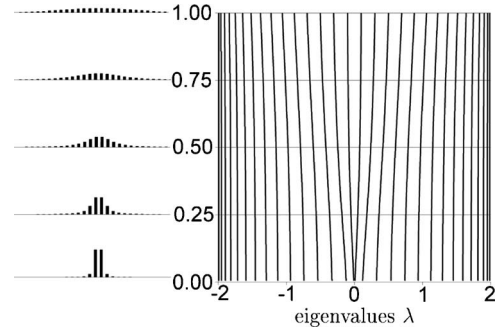
FIG. 4. The dependence of the eigenvalues of H(a) on a (the right-hand side of the figure) and the eigenvector populations \{|\langle v(\lambda)|\Psi(0)\rangle|^2\}_{\lambda} (on the left) for the system of 30 spins.
